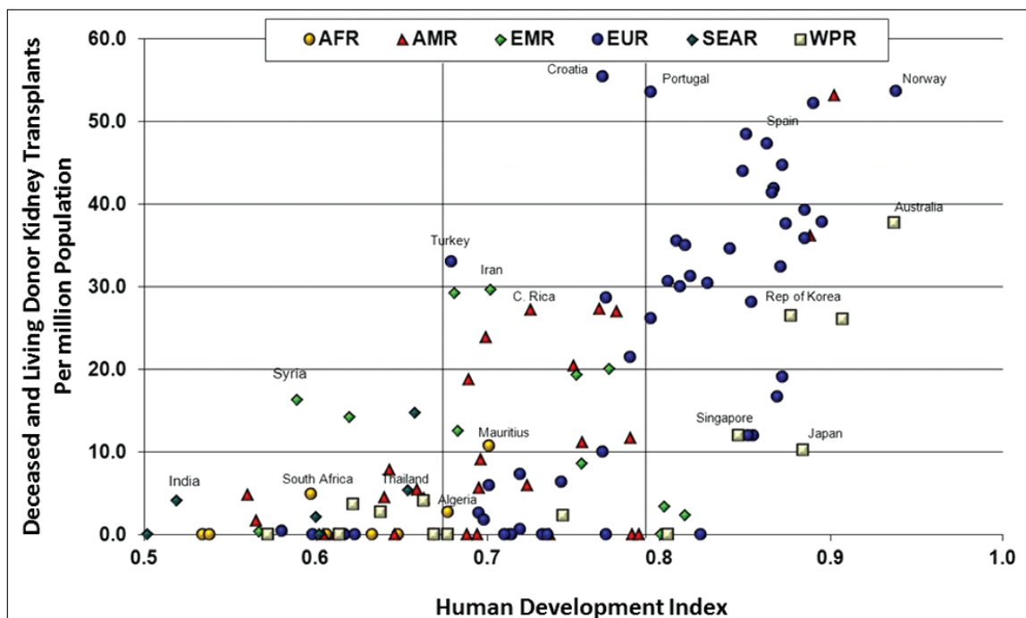
Figure 1: Number of deceased and living donor kidney transplants in World Health Organization member states in 2010, correlated with Human Development Index. Grouped by WHO regions (AFR = Africa, AMR = Americas, EMR = Eastern Mediterranean, EUR = Europe, SEAR = South Eastern Asia, WPR = Western Pacific)
